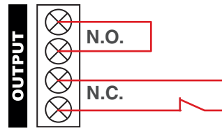
Normal closed mute contact diagram
