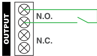
Normal open mute contact diagram
