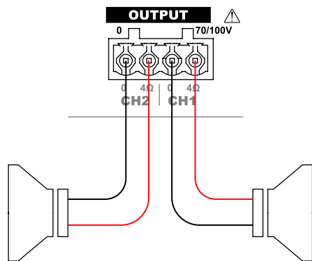
SCP series minimum load impedance in 4 Ohm stereo output mode
